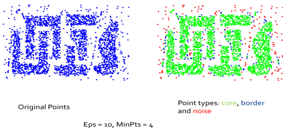
Fig 9. Core point, Border point and Noise point in DBScan
